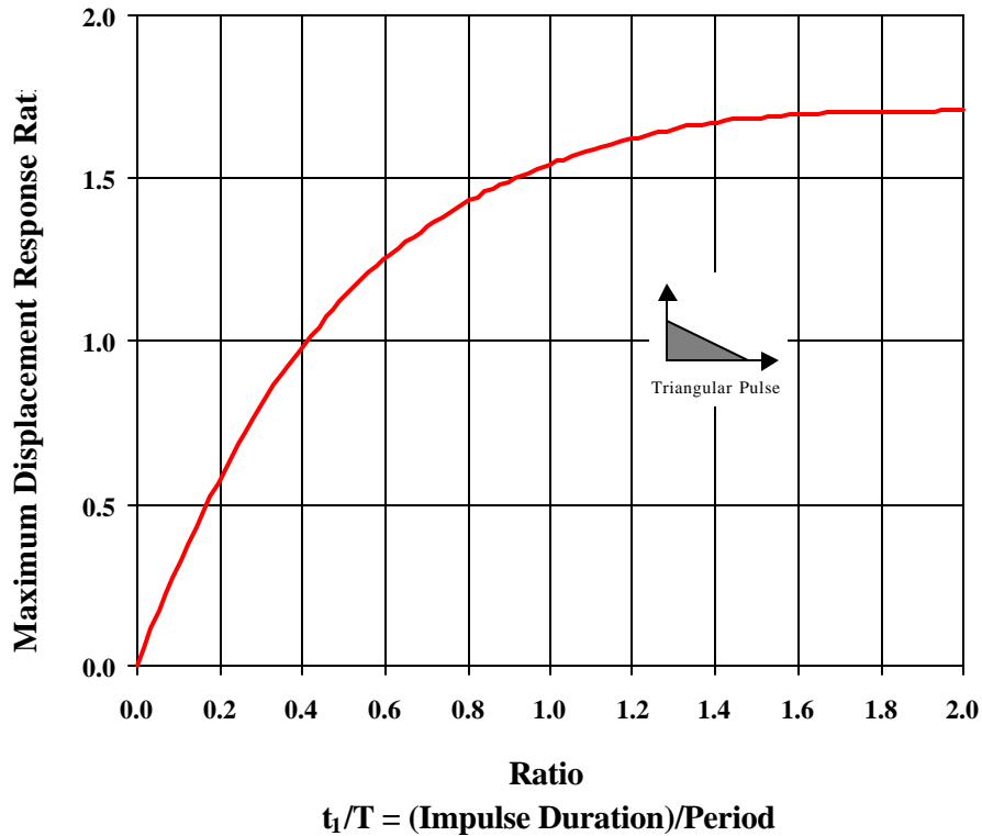
FIGURE 5 SHOCK SPECTRA (CLOUGH & PENZIEN, 1993)
